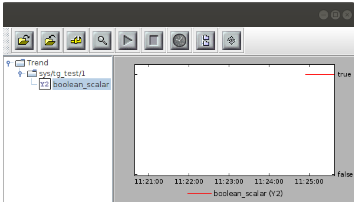
Fig. 14: Boolean trend
