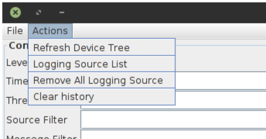
Fig. 24: Actions menu
