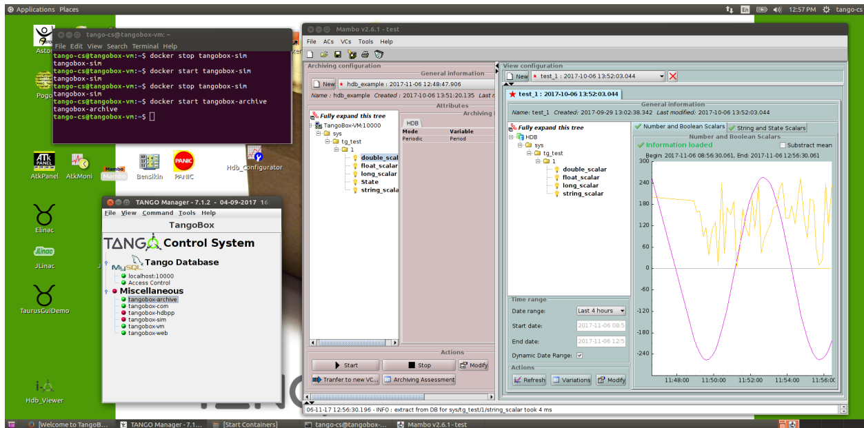
Fig. 5: Screen of running Mambo Please take note of a green bulb of the tangobox-archive node in the Astor window.
