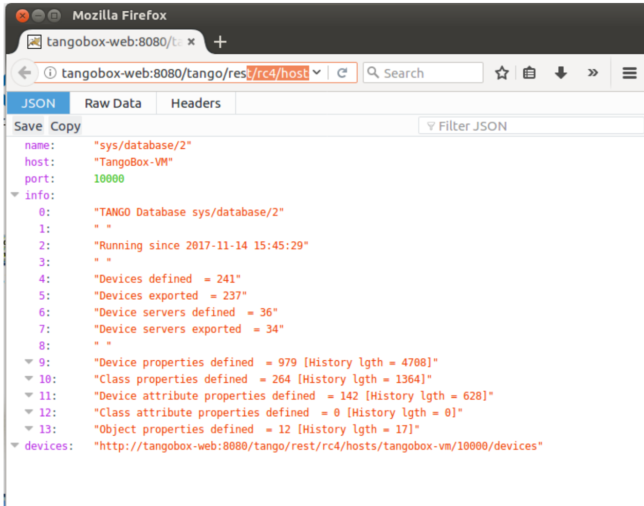
Fig. 8: A web browser window presenting JSON response of the Tango REST server
