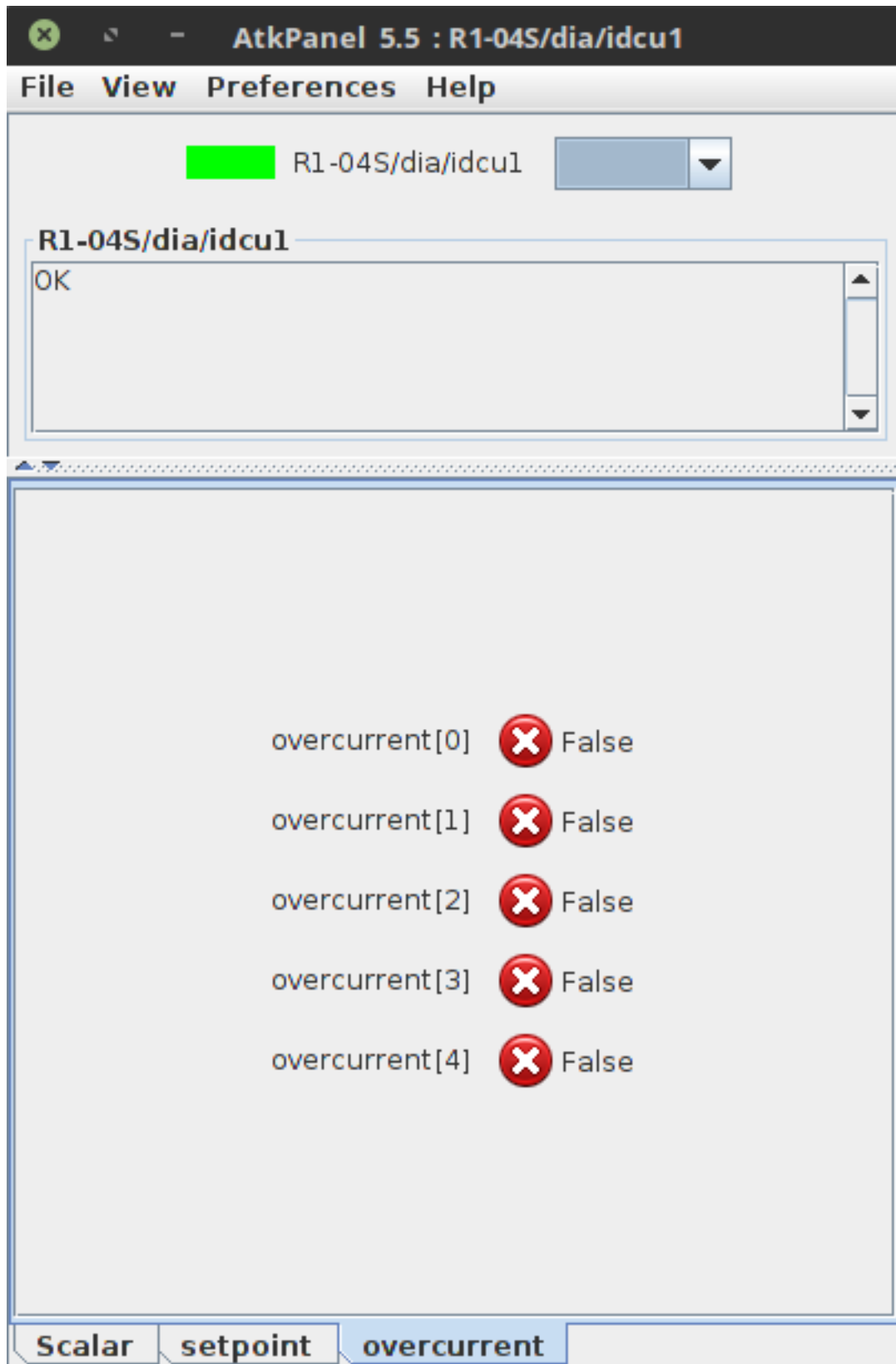
Fig. 6: Boolean array attribute view
