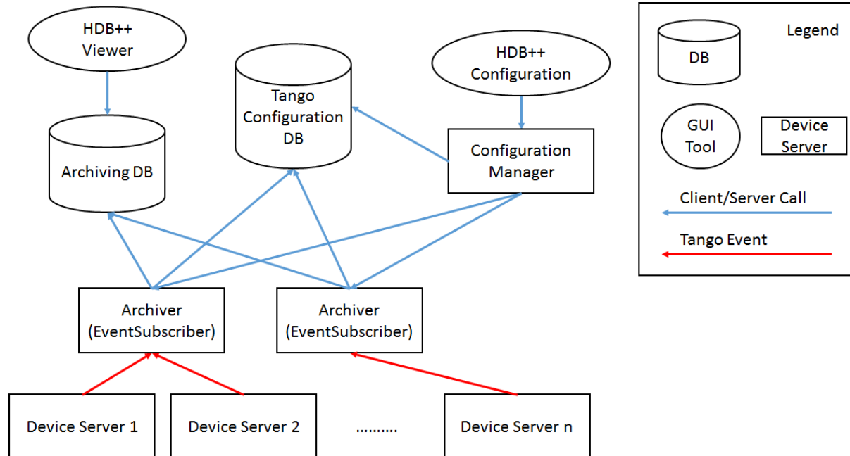
Figure 1: HDB++ Runtime View (part one)
