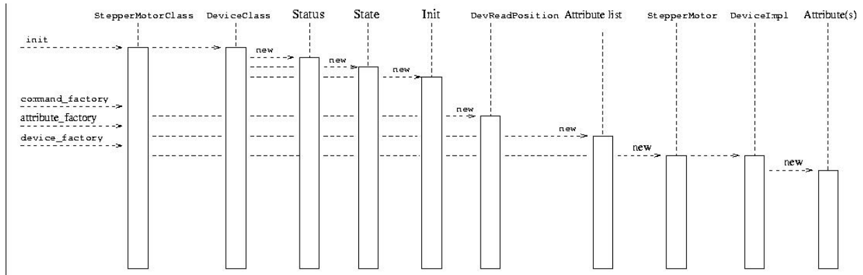
Fig. 7: Figure 6.2: Device pattern startup sequence
