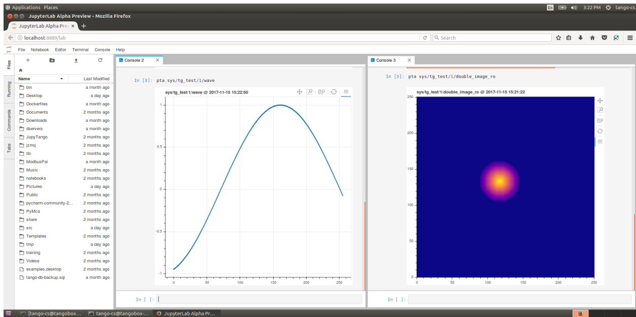
Fig. 3: Browser window with JupyTango in action
