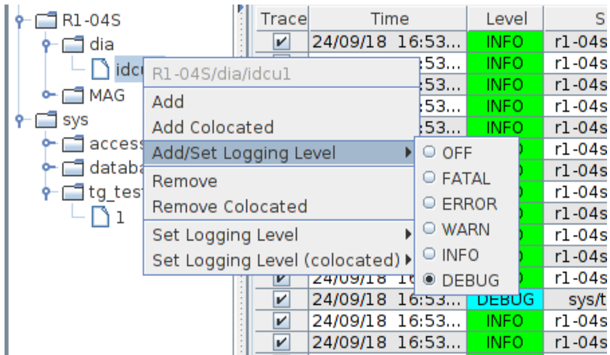
Fig. 23: Add and set logging level
