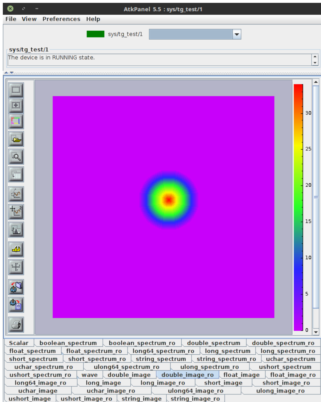
Fig. 7: Image attribute view
