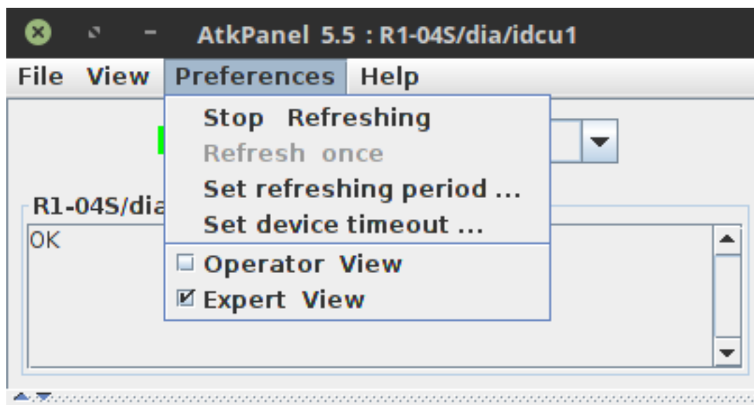
Fig. 20: AtkPanel Preferences
