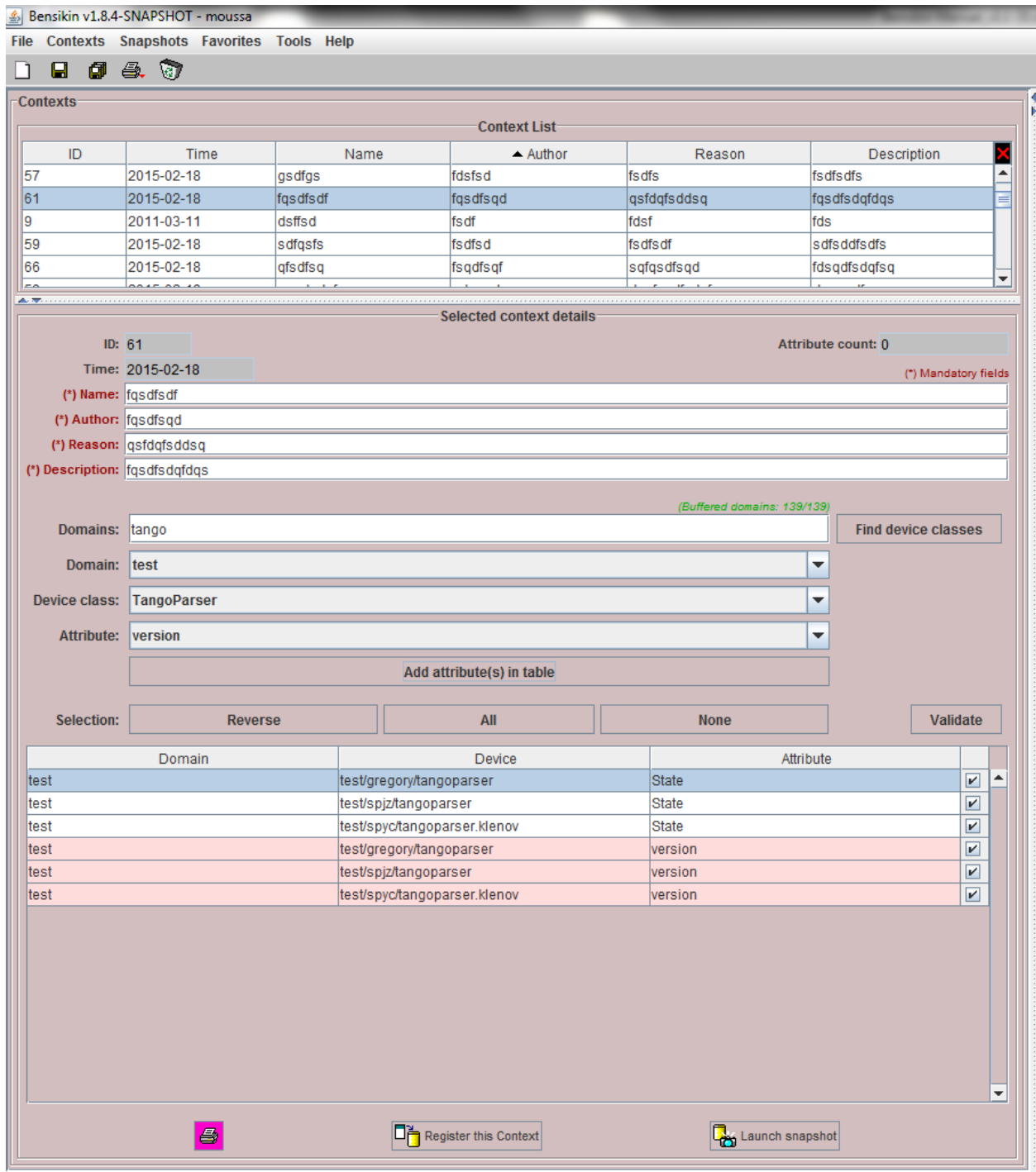
Fig. 34: Figure 10: Bensikin with context table selection mode (modified context)
