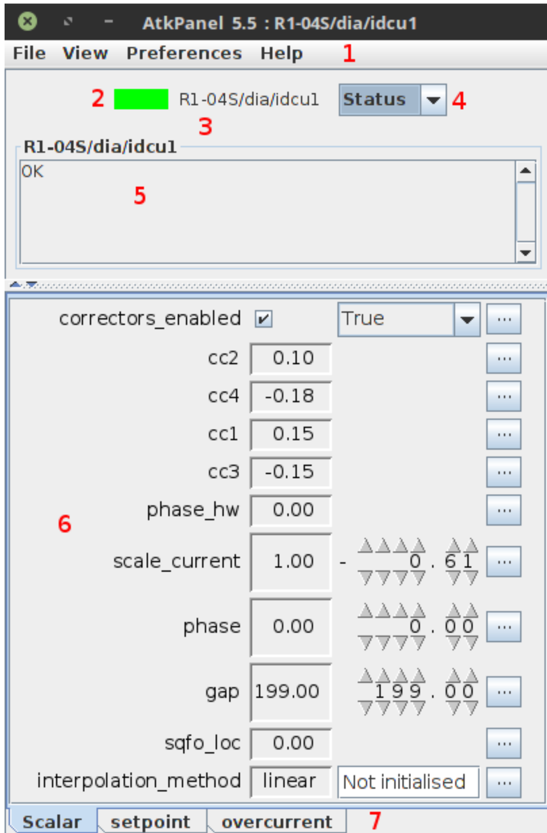
Fig. 3: AtkPanel 5.5 main window
