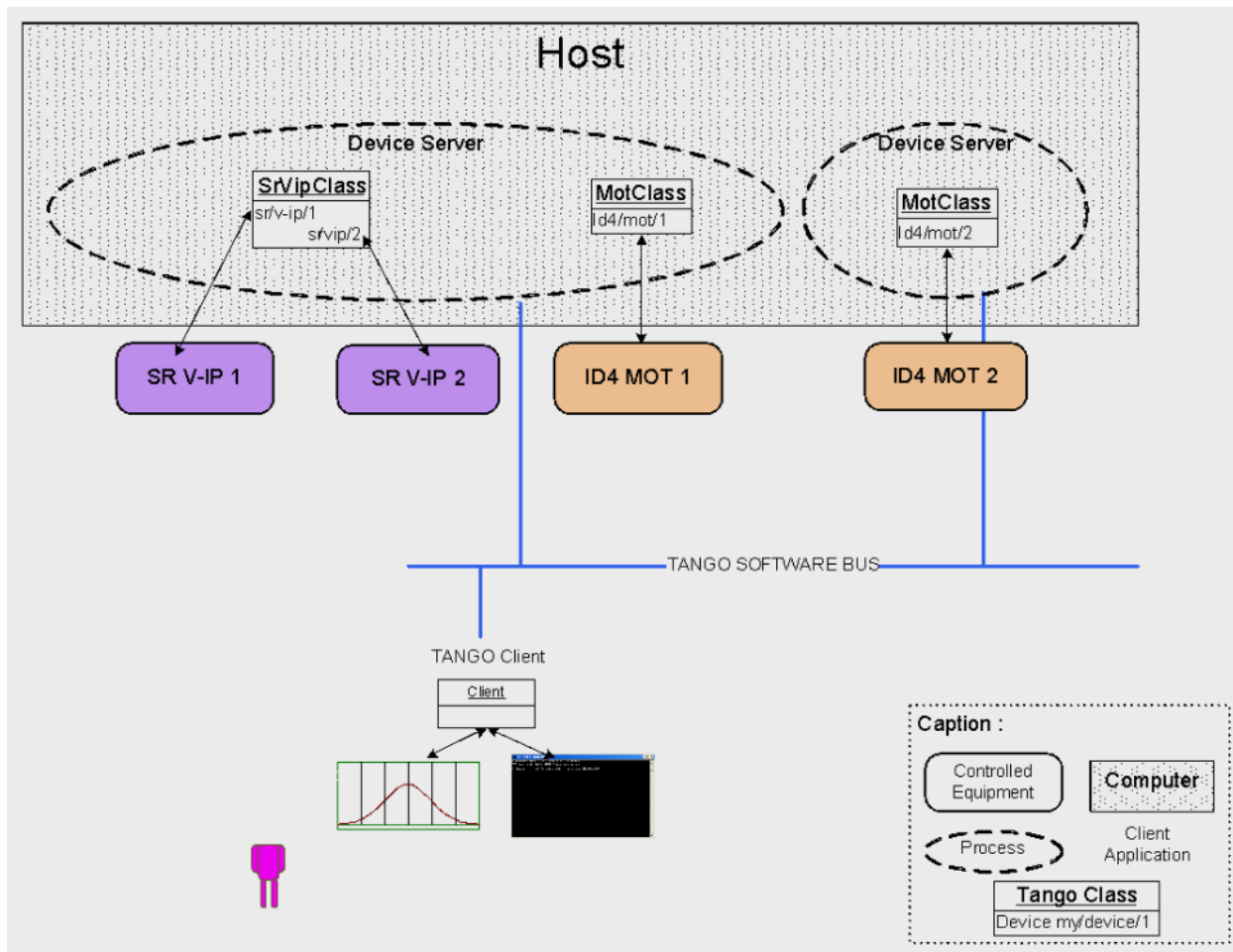
Fig. 4: Tango Deployment
